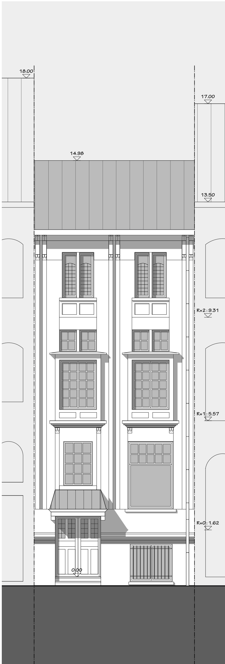
SITUATION EXISTANTE
