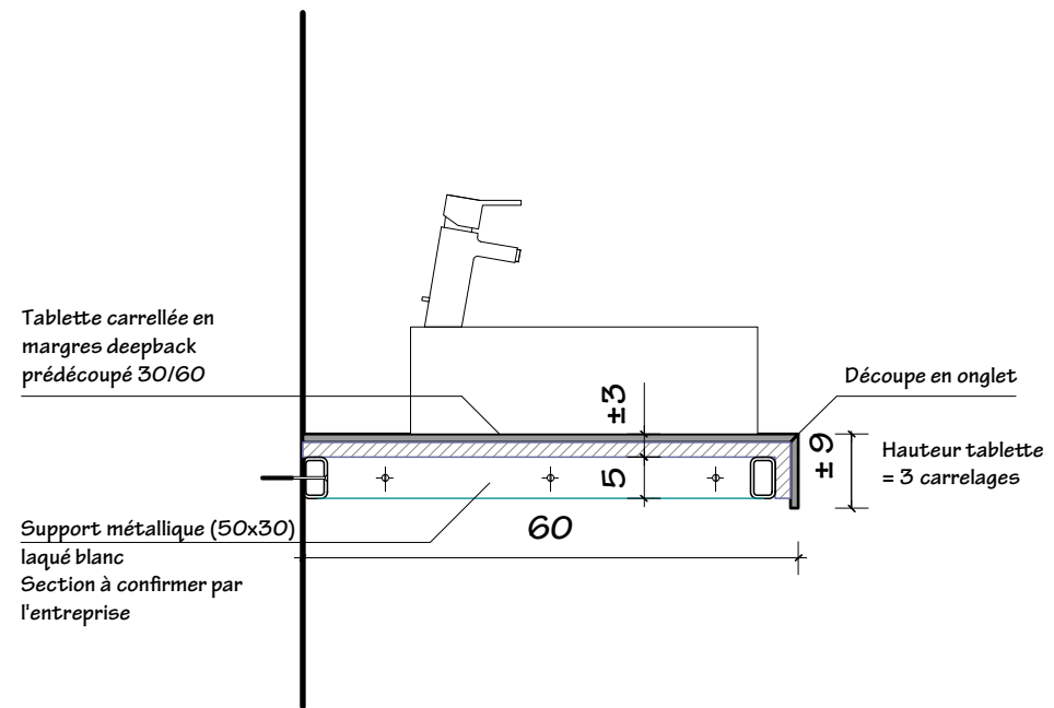
DETAIL FIXATIONS TABLETTE ECH: 1/10
